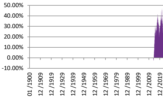
Volatility evolution
